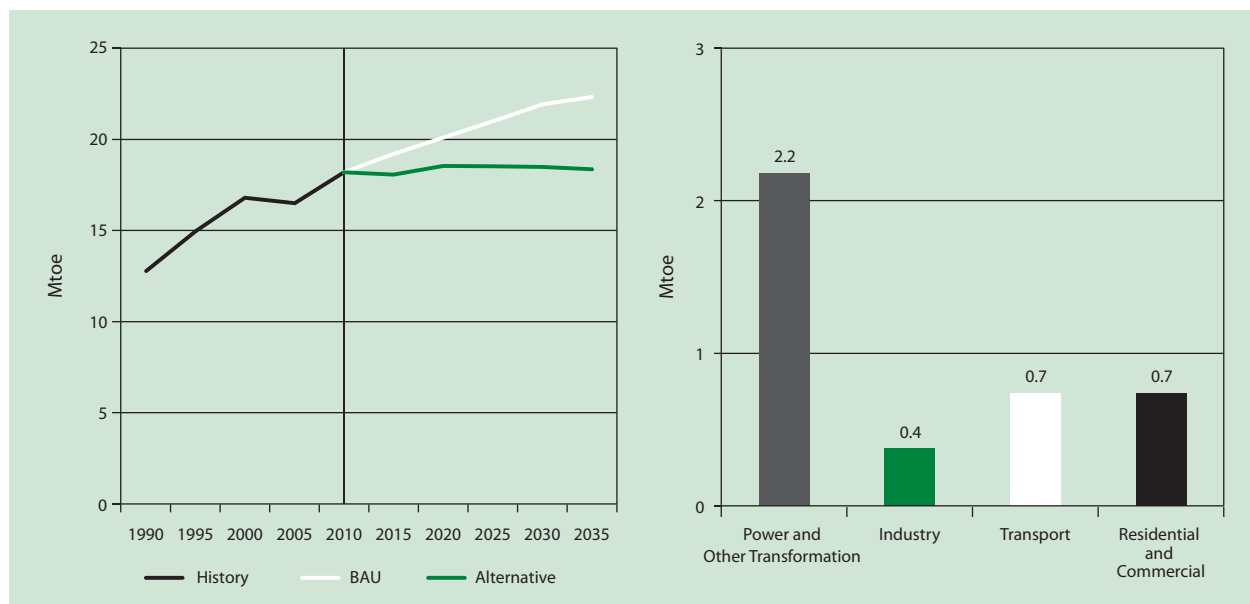
Figure 13.3.4 Comparison of Primary Energy Demand (left) and Sectoral Net Energy Savings in 2035 (right)
